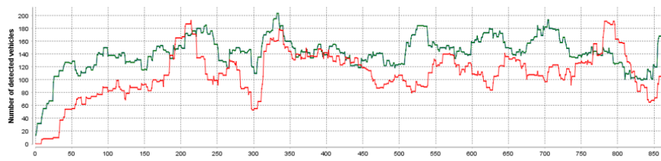
Fig. 6: Traffic flow: number of cars detected by the visual sensors (green) vs number of cars seen by the sensors in the simulation (red) per second.
